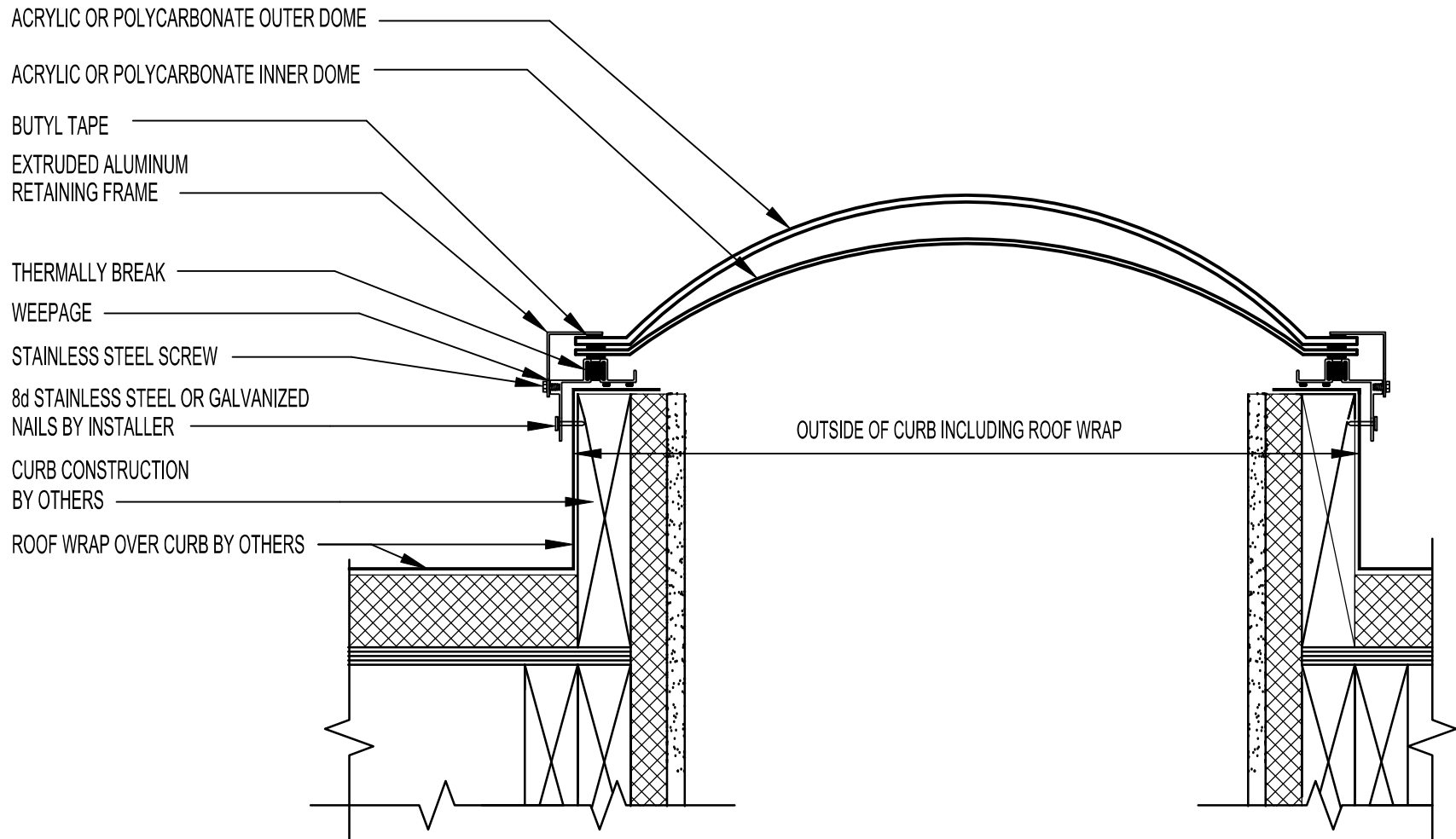
Double Dome Thermal Acrylic/Polycarbonate Skylight, Curb Mount On Site Built Curb
