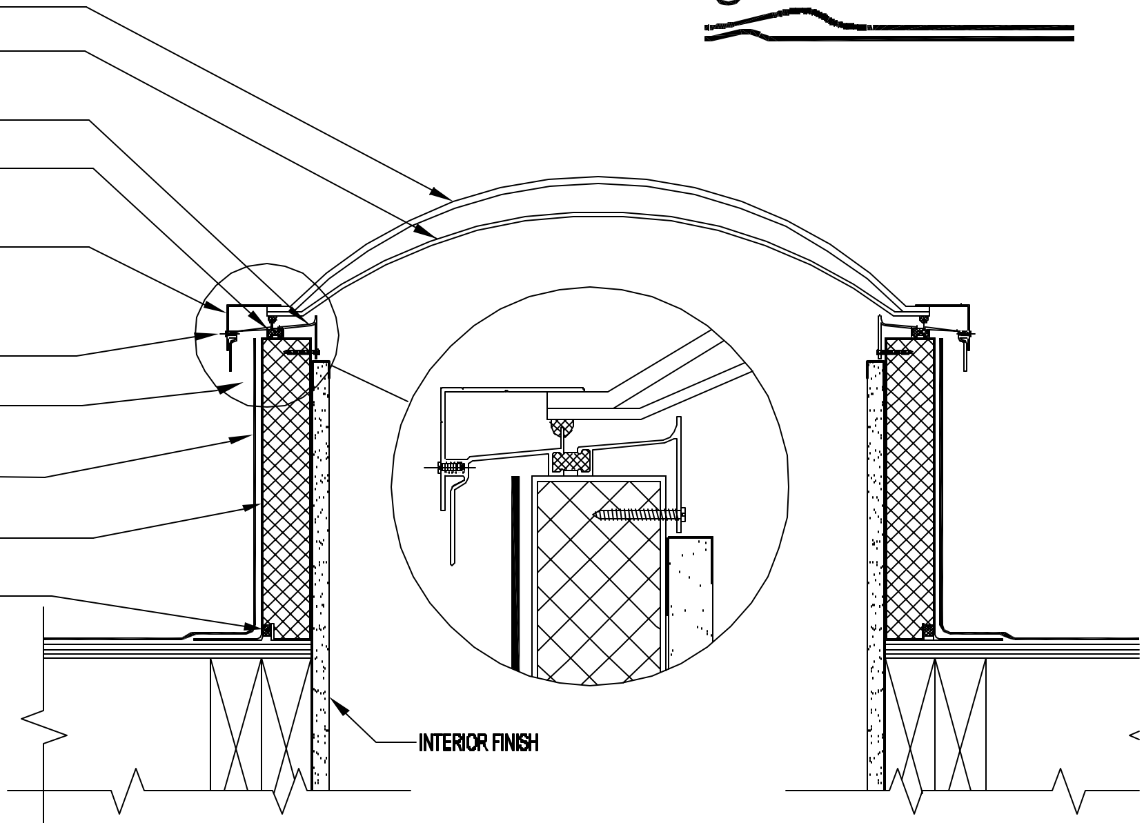
Double Dome Thermal Plastic Skylight With Insulated Integral Roof Mount Curb
